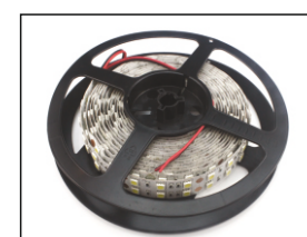
LED Strip: 5050LED, 60LEDs/M, 14.4W/M
